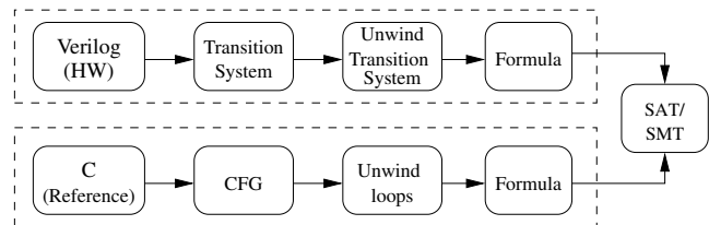
Fig. 1: Equivalence checking tool flow
