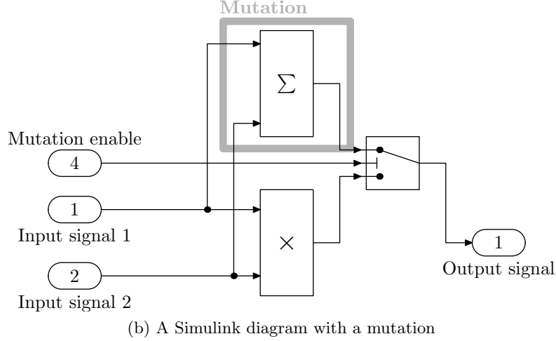
Fig. 4: A simple Simulink program and its mutation
