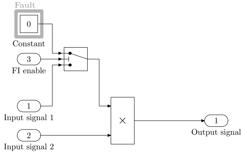
(a) Fault Injection: A signal-stuck-at-0 fault
