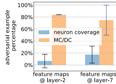
Fig. 3: Adversarial examples detected at each feature map
