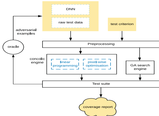
Fig. 1: The DeepConcolic tool
