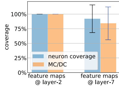
Fig. 2: Coverage results with respect to feature maps
