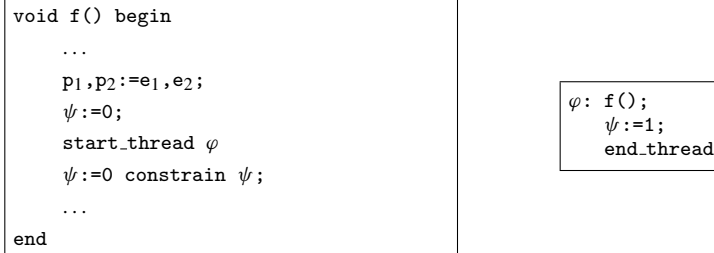
Fig. 5. Over-approximating a recursive call f(e_1, e_2) with thread creation.
